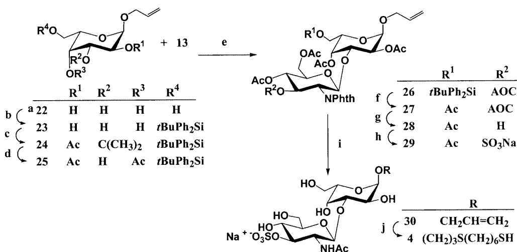
Scheme 4. Reagents and conditions. a, from L-galactose, allyl alcohol, acetyl chloride, 70 °C, 30%; b, t BuPh 2 SiCl, Et 3 N, pyridine, CH 2 Cl 2 , 97%; c, (i) 2,2-dimethoxypropane, p TsOH, DMF; (ii) acetic anhydride, pyridine, 60% over two reaction steps. d, (i) TFA, water, CH 2 Cl 2 ; (ii) trimethyl orthoacetate, p TsOH, CH 2 Cl 2 ; (iii) acetic acid, water, 40 °C, 78% over three reaction steps. e, acceptor 25 , donor 13 , TMSOTf, CH 2 Cl 2 , 98%; f, (i) 1 M tetrabutylammonium fluoride in THF, acetic acid, pH 7, 0 °C; (ii) acetic anhydride, pyridine, 84% over two reaction steps. g, [Pd(PPh 3 ) 4 ], morpholine, THF, 65 °C, 96%; h, SO 3 ·NMe 3 , DMF, 50 °C, 82%; i, (i) 33% NH 2 Me in ethanol, 5 days; (ii) acetic anhydride, MeOH, 0 °C, 96% over two reaction steps. j, 1,6-hexanedithiol, UV light, MeOH, 60%. (AOC = COOCH 2 CH=CH 2 ; t BuPh 2 Si = (CH 3 ) 3 CSi(C 6 H 5 ) 2 )
