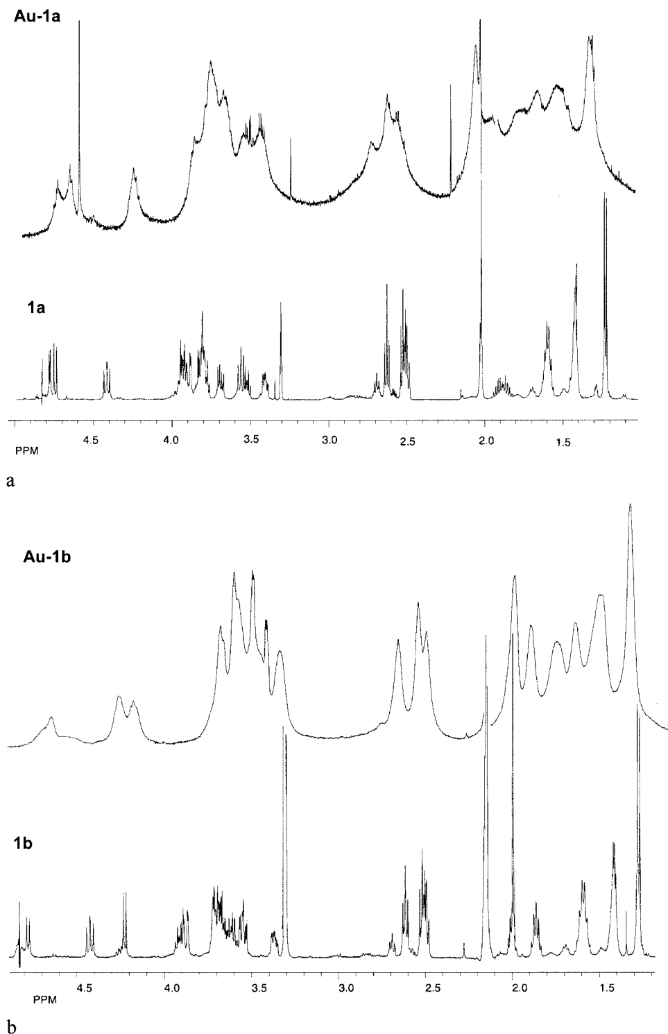
Figure 2. a : Comparison of the 1 H NMR spectra of gold glyconanoparticles Au-1a (in D 2 O) and thiol spacer containing disaccharide 1a (in CD 3 OD). b : Comparison of the 1 H NMR spectra of gold glyconanoparticles Au-1b (in D 2 O) and thiol spacer containing disaccharide 1b (in CD 3 OD)
