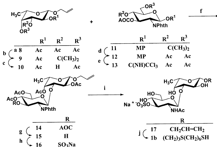
Scheme 2. Reagents and conditions. a, (i) from L-fucose tetraacetate, 33% HBr/HOAc, 0 °C; (ii) allyl alcohol, Hg(CN) 2 , 95% over two reaction steps. b, (i) NaOMe, MeOH; (ii) 2,2-dimethoxypropane, p TsOH, DMF; (iii) acetic anhydride, pyridine, 80% over three reaction steps. c, (i) TFA, water, CH 2 Cl 2 ; (ii) trimethyl orthoacetate, p TsOH, CH 2 Cl 2 ; (iii) acetic acid, water, 40 °C, 51% over three reaction steps. d, (i) TFA, water, CH 2 Cl 2 ; (ii) acetic anhydride, pyridine, quantitative overall yield. e, (i) ammonium cerium(IV) nitrate, acetonitrile/toluene/water (1:1:1); (ii) trichloroacetonitrile, 1,8-diazabicyclo[5.4.0]undec-7-ene, CH 2 Cl 2 , 47% over two reaction steps. f, donor 13 , acceptor 10 , TMSOTf, CH 2 Cl 2 , 69%. g, [Pd(PPh 3 ) 4 ], morpholine, THF, 65 °C, 65%. h, SO 3 ·NMe 3 , DMF, 50 °C, 89%. i, (i) 33% NH 2 Me in EtOH, 5 days; (ii) acetic anhydride, MeOH, 0 °C, 87% over two reaction steps. j, 1,6-hexanedithiol, UV light, MeOH, 83%. (AOC = COOCH 2 CH=CH 2 ; MP = C 6 H 4 OCH 3 )
