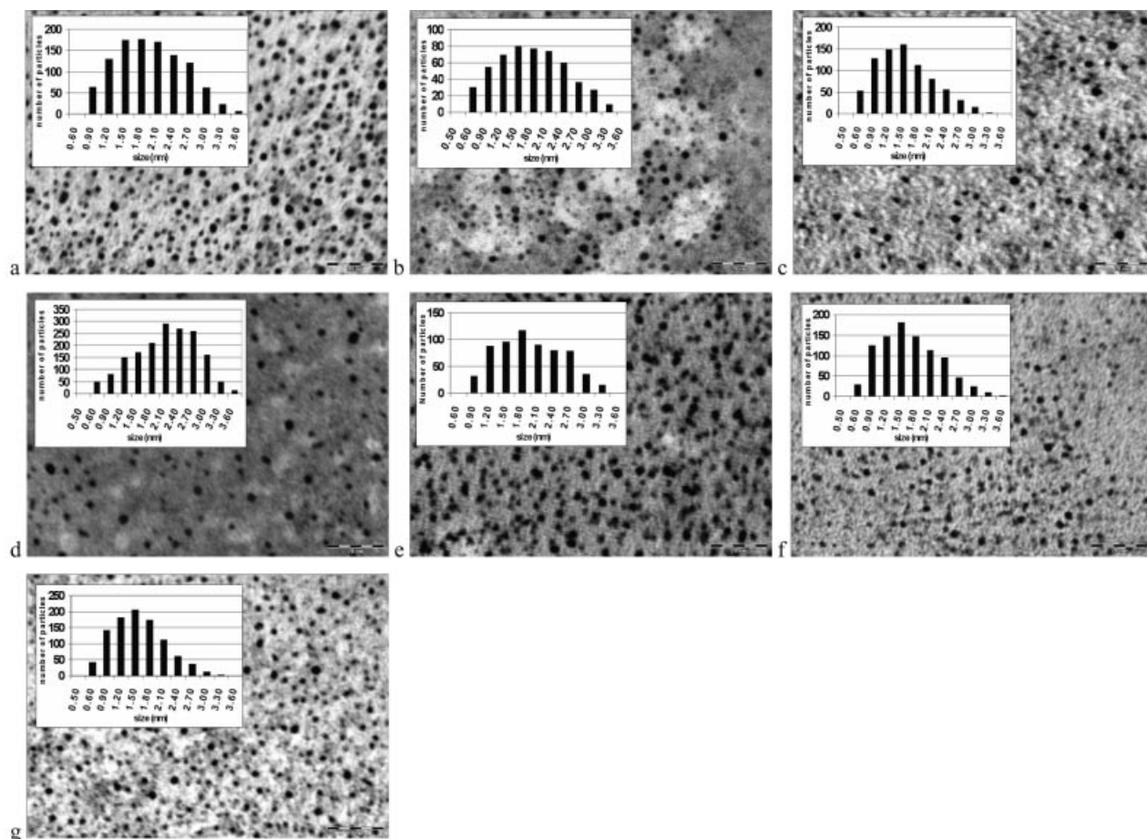
Figure 3. TEM images of Au-1a/b to Au-6 in water ( 0.1 \text{ mg}\cdot\text{mL}^{-1} ); scale bars 20 nm. a, Au-1a . b, Au-1b . c, Au-2 . d, Au-3 . e, Au-4 . f, Au-5 . g, Au-6 . Inserts: Particle size distributions
