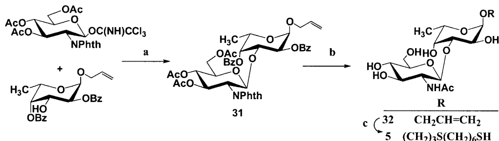
Scheme 5. Reagents and conditions. a, acceptor, donor, TMSOTf, \text{CH}_2\text{Cl}_2 , 86%. b, (i) ethylenediamine, n\text{BuOH} , 90 °C; (ii) acetic anhydride, pyridine; (iii) NaOMe, MeOH, 80% over three reaction steps. c, 1,6-hexanedithiol, UV light, MeOH, quantitative. (Bz = \text{COC}_6\text{H}_5 )
