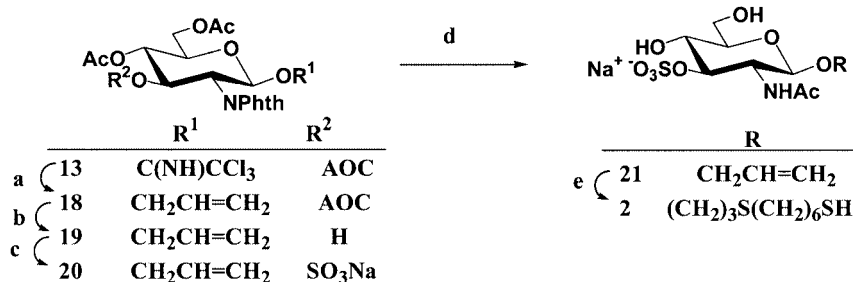
Scheme 3. Reagents and conditions. a, allyl alcohol, TMSOTf, CH 2 Cl 2 , 45%; b, [Pd(PPh 3 ) 4 ], morpholine, THF, 50 °C, quantitative; c, SO 3 ·NMe 3 , DMF, 50 °C, 39%; d, (i) 33% NH 2 Me in ethanol, 5 days; (ii) acetic anhydride, MeOH, 0 °C, 66% over two reaction steps. e, 1,6-hexanedithiol, UV light, MeOH, 42%. (AOC = COOCH 2 CH=CH 2 )
