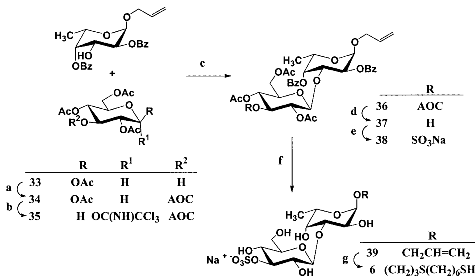
Scheme 6. Reagents and conditions. a, allyl chloroformate, pyridine, \text{CH}_2\text{Cl}_2 , -30 °C, quantitative. b, (i) \text{NH}_2\text{NH}_2 \cdot \text{HOAc} , DMF; (ii) trichloroacetonitrile, 1,8-diazabicyclo[5.4.0]undec-7-ene, \text{CH}_2\text{Cl}_2 , 60% over two reaction steps. c, donor 35 , acceptor, TMSOTf, \text{CH}_2\text{Cl}_2 , 60%. d, [\text{Pd}(\text{PPh}_3)_4] , morpholine, THF, 65 °C, 93%. e, \text{SO}_3 \cdot \text{NMe}_3 , DMF, 50 °C, 53%. f, NaOMe, MeOH, quantitative. g, 1,6-hexanedithiol, UV light, MeOH, 50%. (AOC = \text{COOCH}_2\text{CH}=\text{CH}_2 ; Bz = \text{COC}_6\text{H}_5 )
