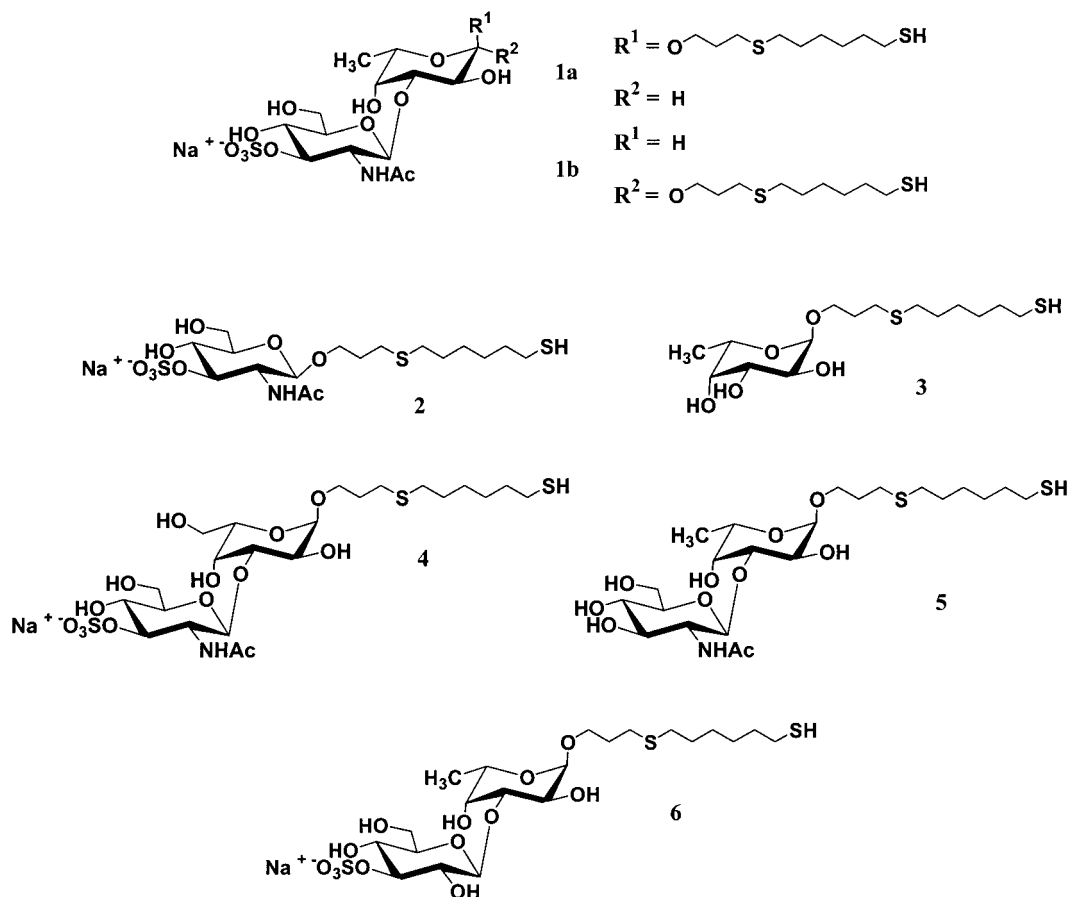
Figure 1. Target structures 1a/b to 6 containing a thiol spacer
